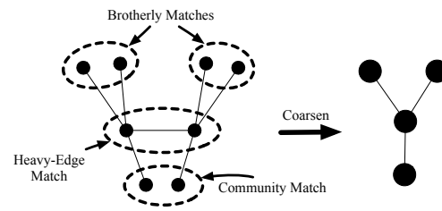
Figure 3: Community Matching
