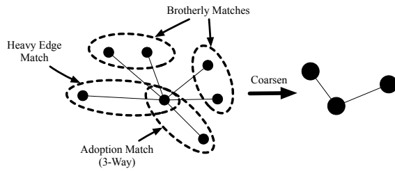
Figure 2: Brotherly Matching
